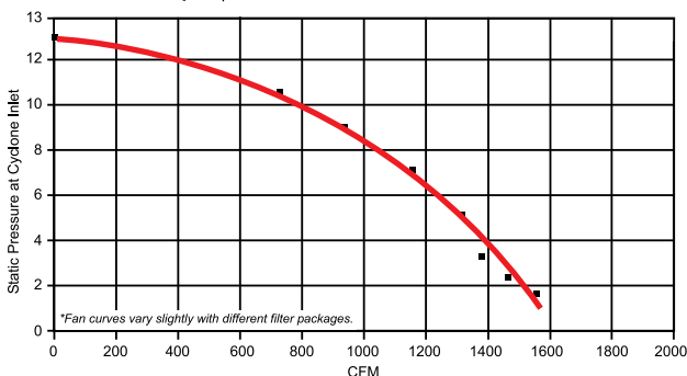
3hp Super Dust Gorilla CFM vs. SP Curve*
